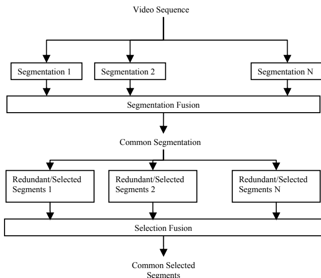
Figure 1: Overview of the collaborative summarization process.
