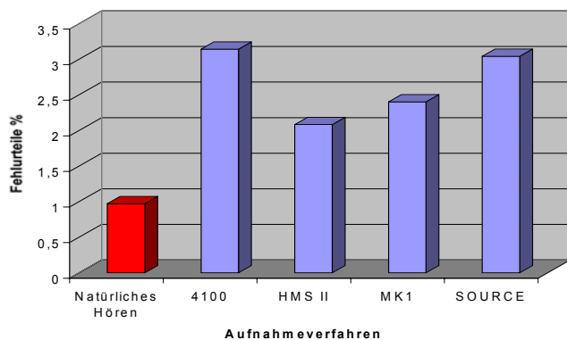
Abb. 2 Out-of-cone errors
