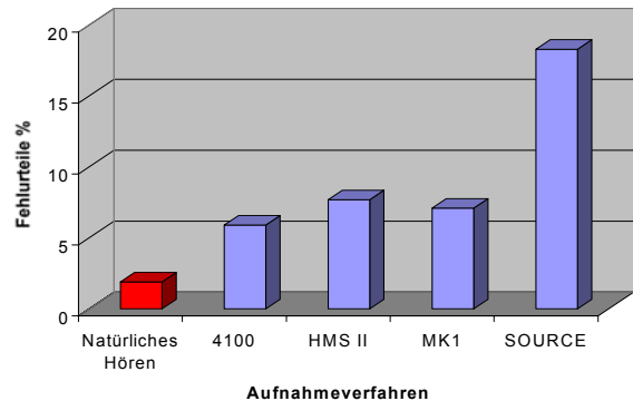
Abb. 3 Within-cone errors
