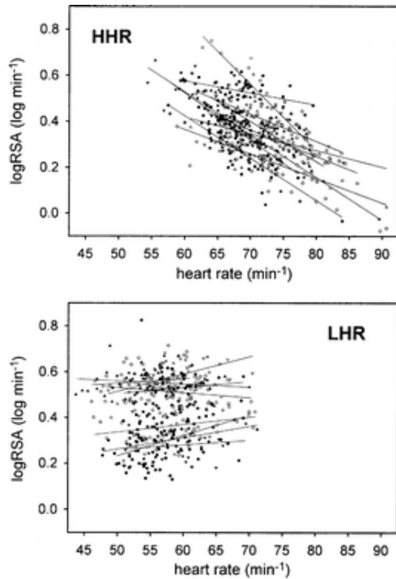
Fig. 5. Linear correlation between daily values of HR and logRSA within the individual women of the HHR group (top graph) and the LHR group (bottom graph)
