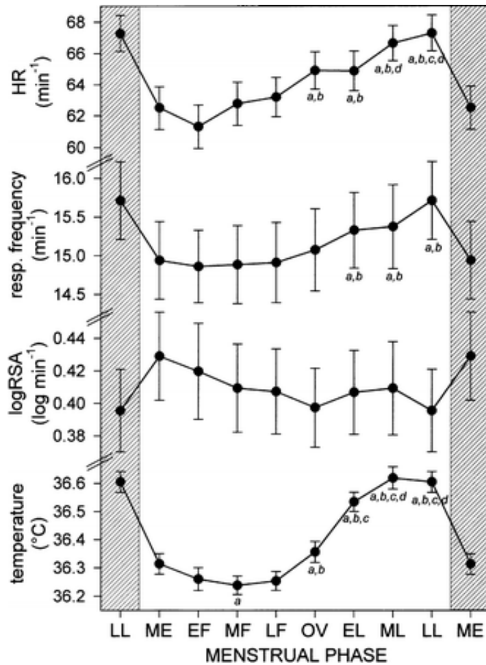
Fig. 2. Heart rate ( HR ), respiratory ( resp. ) frequency, time-domain measure of respiratory sinus arrhythmia ( logRSA ) and basal body temperature during the eight phases of the menstrual cycle [mean values (SEM)] of all subjects ( n=26 ). To emphasize the cyclic pattern, the first and the last menstrual phase (ME and LL) are plotted twice (shaded areas). a Significantly different from menstrual phase (ME); b significantly different from all follicular phases (EF, MF, LF), c significantly different from ovulatory phase (OV), d significantly different from early luteal phase (EL)
