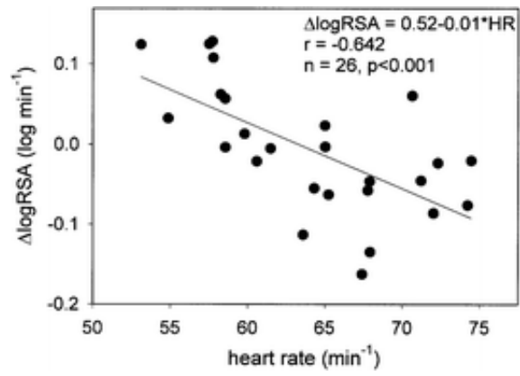
Fig. 3. Difference between the extreme values of logRSA ( \Delta \log RSA ; ML minus EF phase) as a function of average HR in 26 subjects
